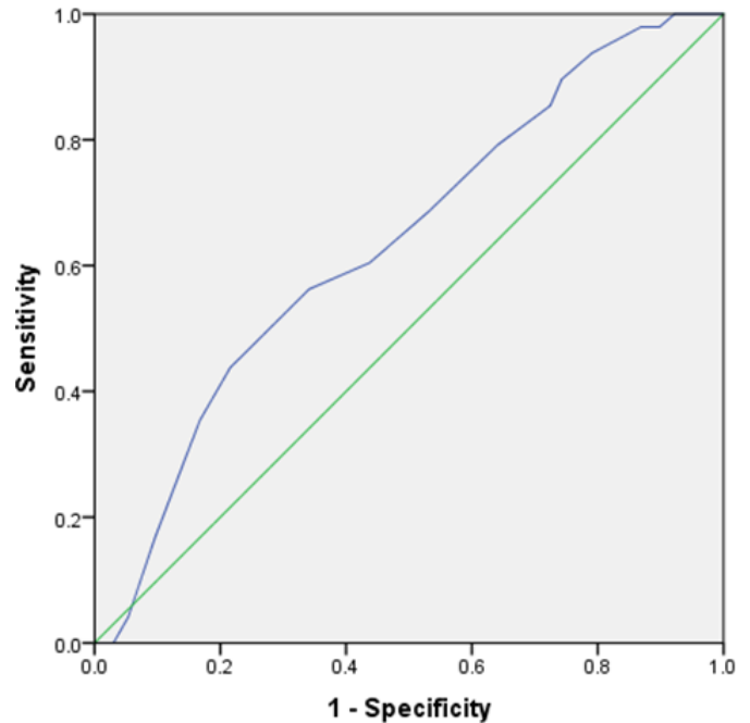
Figure 3 Receiver operating characteristic curves of 30-s chair-stand test (CS-30) as an indicator of sedentary lifestyle in women. CS-30 optimal cut-off: \leq 21 . Sensitivity: 0.854. Specificity: 0.275. Area under the curve: 0.637.
